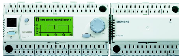
Synco™ 700 control with attached extension module RMZ78...
