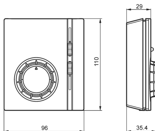
Room thermostat
