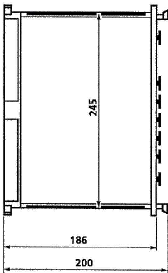
Device dimensions
